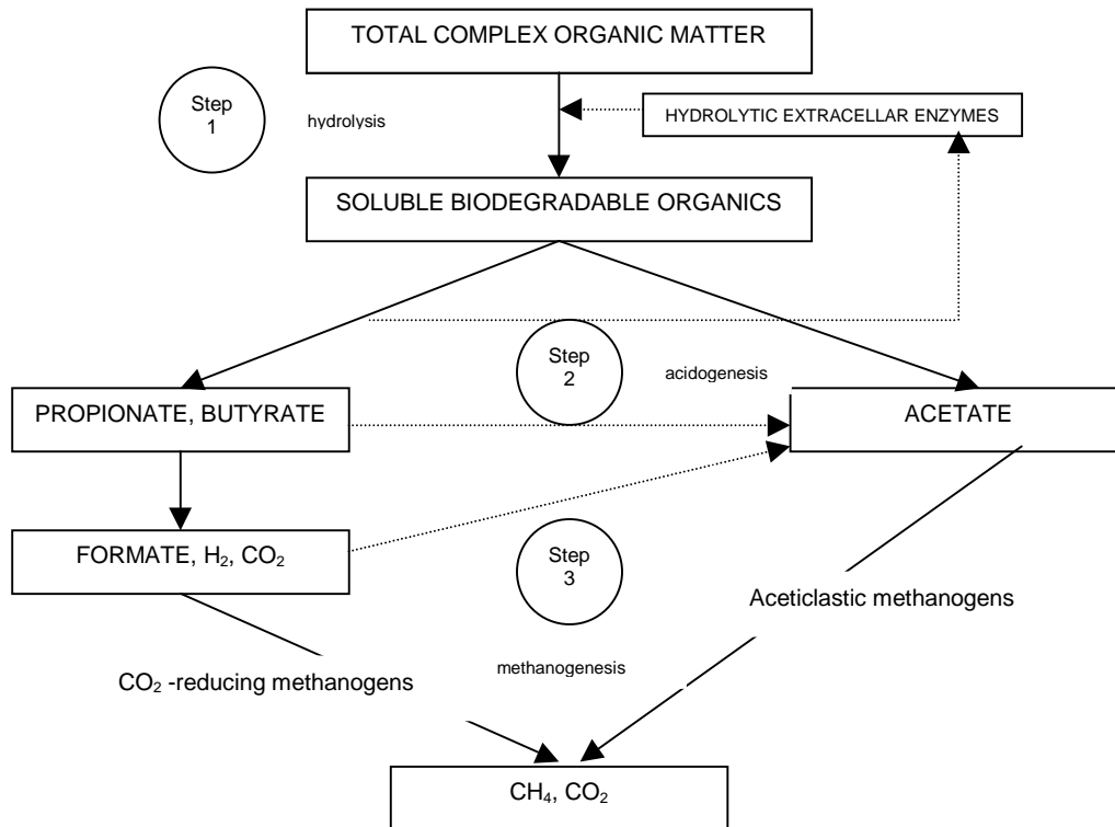
Figure 2-1 Anaerobic digestion of organic matter and methane production (After Hill et al., 1987)
