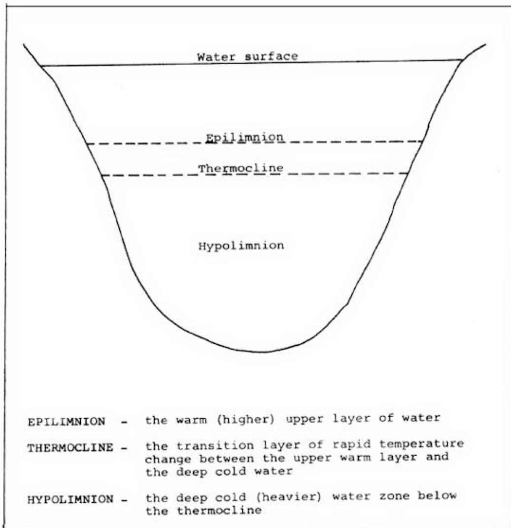
Figure 2: Section of Riley Lake showing the three layers resulting from thermal stratification.
