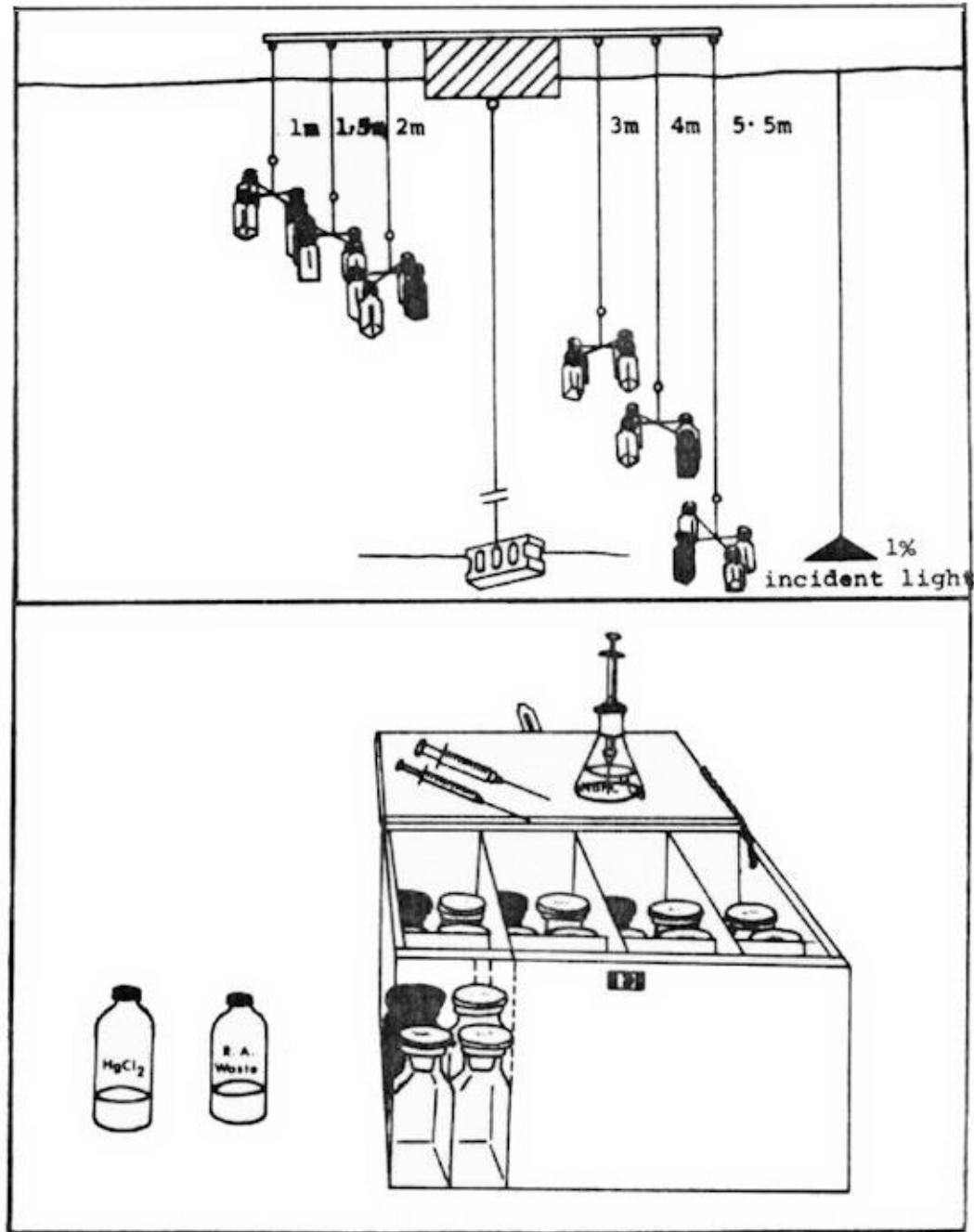
Figure 4. Diagrammatic representation (a) for determining photosynthetic activity of photic zone and (b) of field equipment: 10 ml syringe; 25 ml syringe; 1 ml syringe and sterile 14 C reservoir; light and dark bottles; HgCl 2 and container for radioactive waste material.
