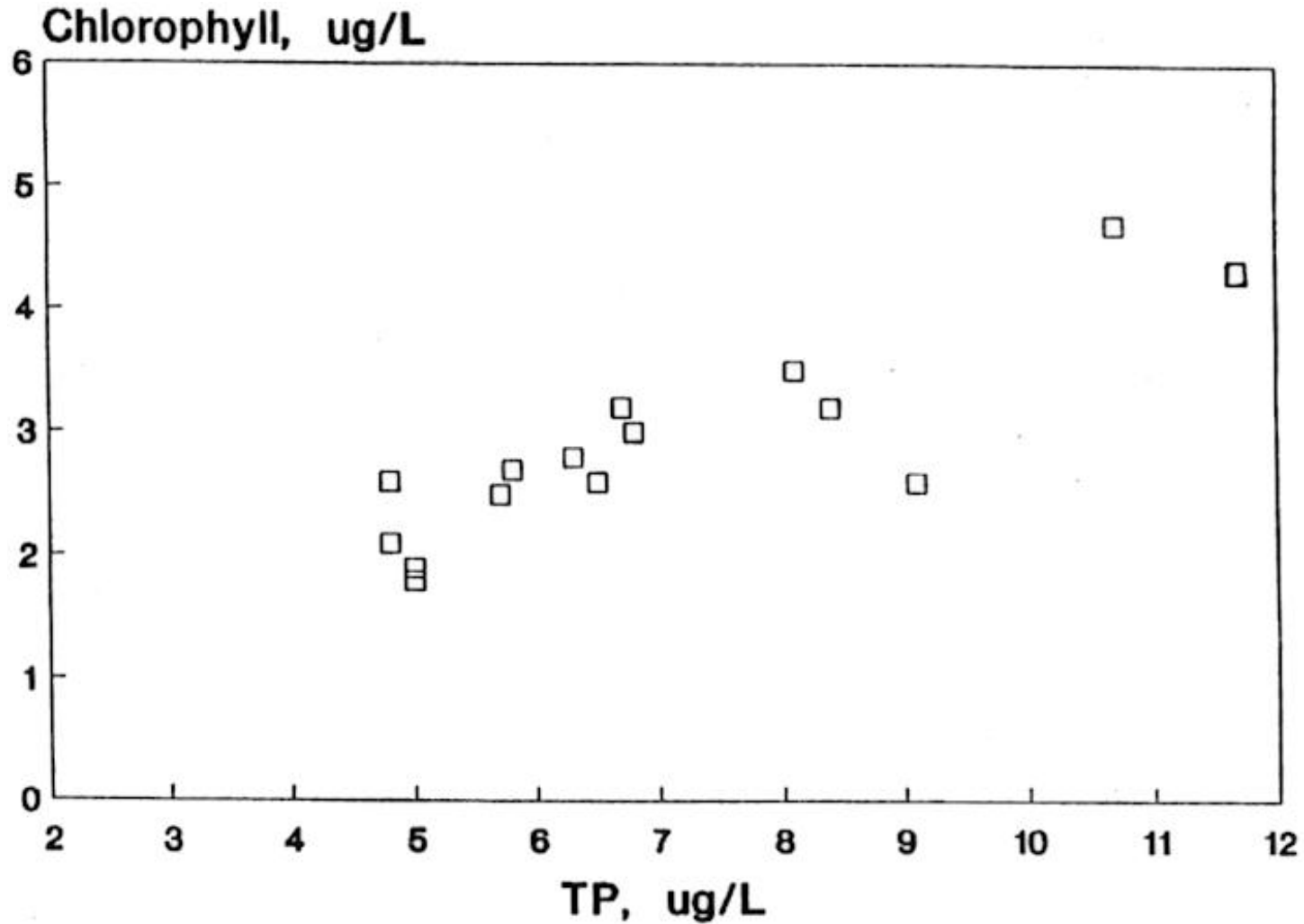
Figure 1(a). Ice-free chlorophyll a versus epilimnetic TP for 15 P-limited lakes in central Ontario for the 12 year period 1976-1987. Average of annual means. The regression equation is Chl_{if} = 0.332 TP + 0.571 ( n = 15 , R^2 = 0.78 , slope SE = 0.049 and the intercept SE = 0.358).
