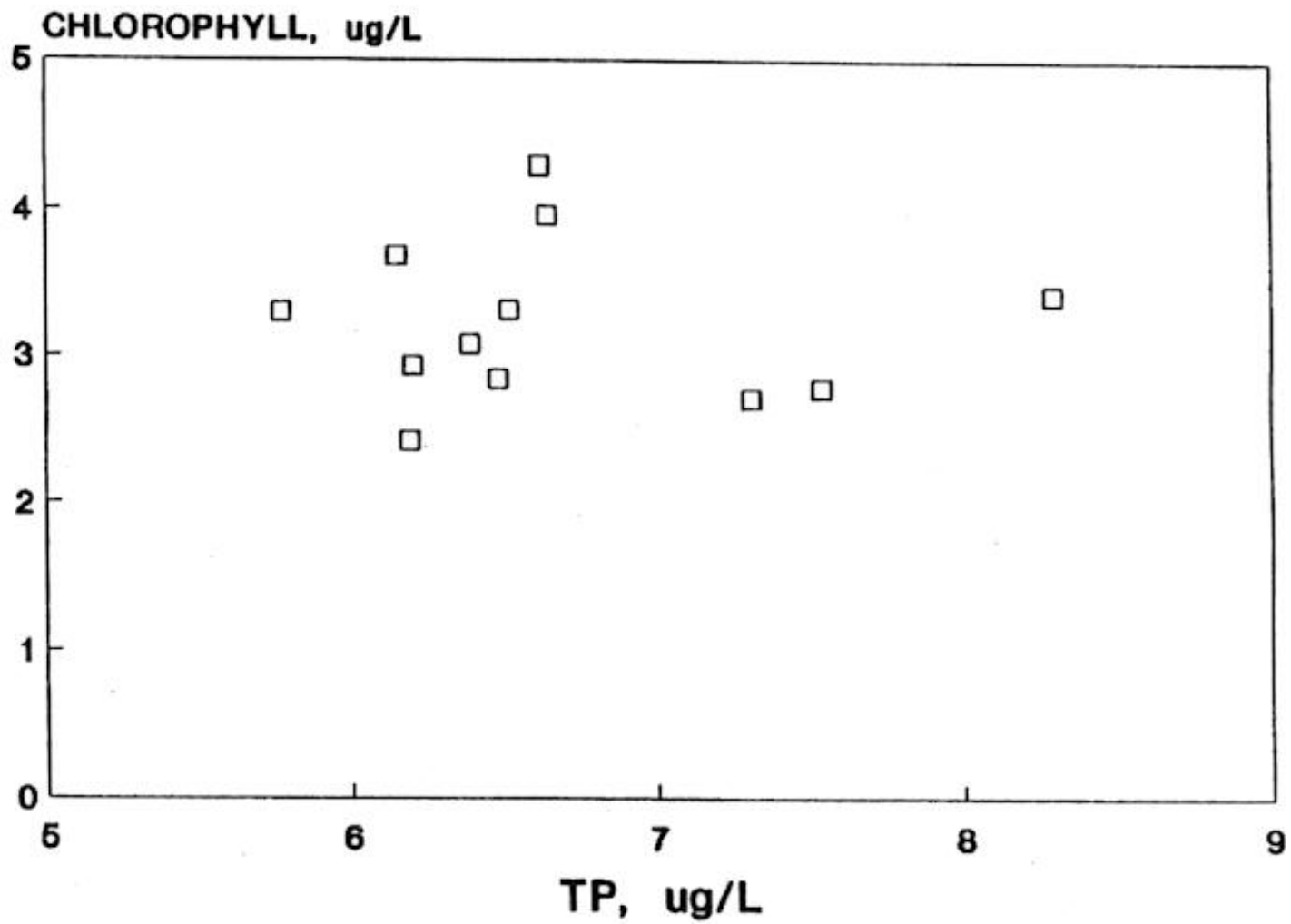
Figure 2(a). Annual ice-free chlorophyll a versus epilimnetic TP for Harp Lake 1976 - 1987.
