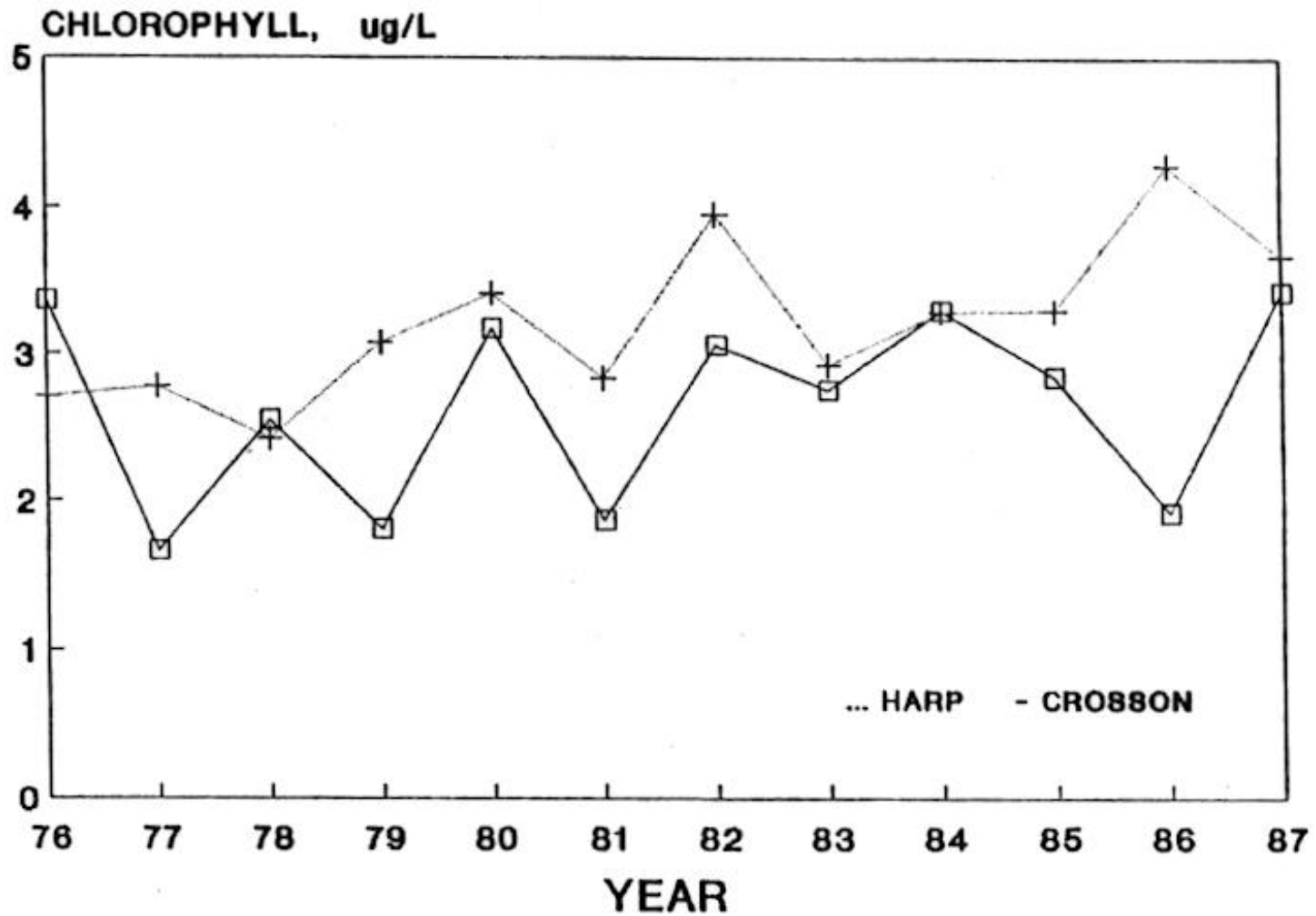
Figure 3(a). Temporal responses of annual ice-free chlorophyll a in Harp and Crosson Lakes from 1976 to 1987.
