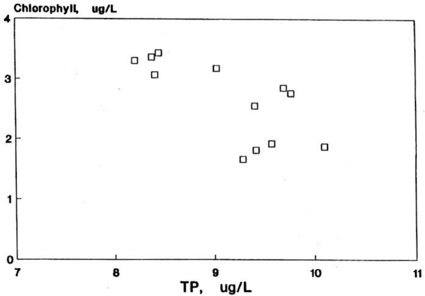
Figure 2(b). Annual ice-free chlorophyll a versus epilimnetic TP for Crosson Lake, 1976 - 1987.
