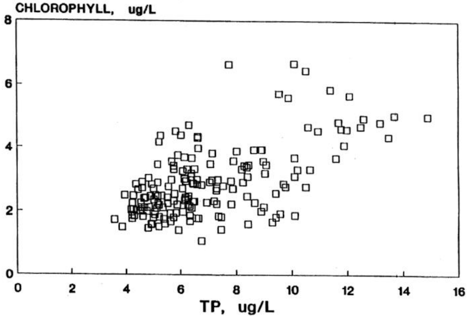
Figure 1(b). Ice-free chlorophyll versus epilimnetic TP for 15 P-limited lakes in central Ontario for the 12 year period 1976-1987. Annual means ( n = 172 lake-years, R^2 = 0.36 ).
