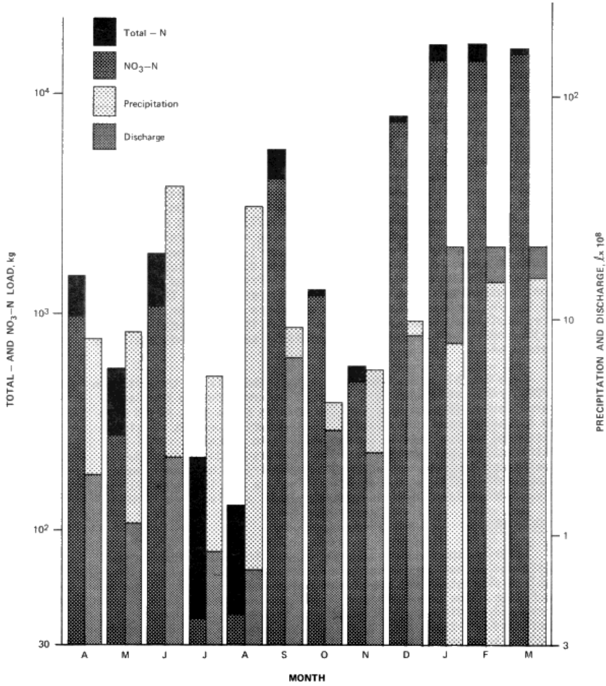
Figure 3. Monthly total — and NO 3 —N load, precipitation, and discharge at the site downstream of highway 3 on Hillman Creek.
