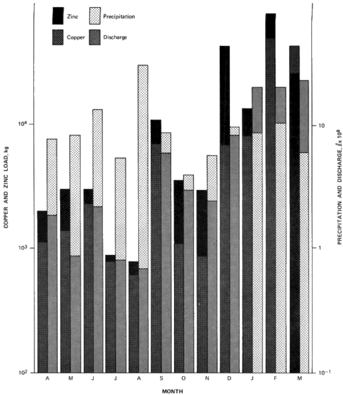
Figure 6. Monthly copper, and zinc load, precipitation, and discharge at the site downstream of highway 3 on Hillman Creek.
