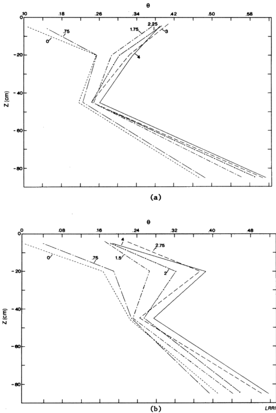
Fig. 12-16: Volumetric water content ( \theta ) versus depth ( Z ) profiles obtained during infiltration at site #4 in Watershed AG-1. The parameter labelling each line is the time, in hours, from the beginning of infiltration. (a) The data points plotted at Z = -5, -20, -45, -85 are means of six measurements made in soil away from cracks. (b) similar to (a) except measurements were made about 5 cm from cracks.
