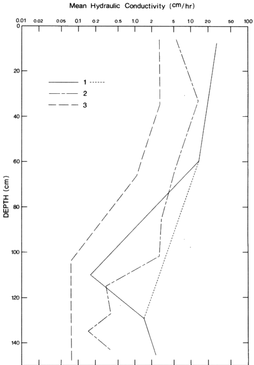
Fig. 12-4: Geometric mean hydraulic conductivities versus depth for the three sites in Watershed AG
