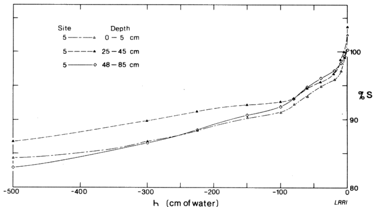
Fig. 12-13: Mean desorption soil water capacity relationships for site #5 in Watershed AG-1. The degree of saturation, as a percentage, was plotted against pressure head ( h ) for three depth intervals to 85 cm.
