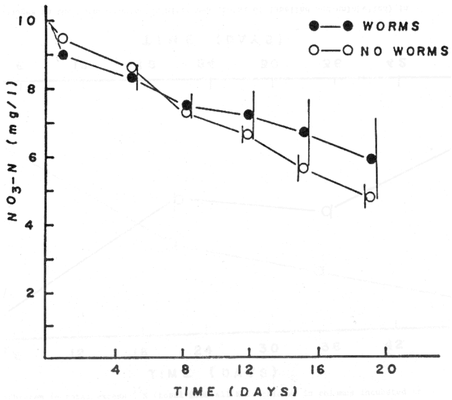
Figure 8: Changes in nitrate-N concentration in the nitrate solution overlying 10 cm of Canagagigue sediment when fresh nitrate was added. Mean of 3 replicates \pm SD.
