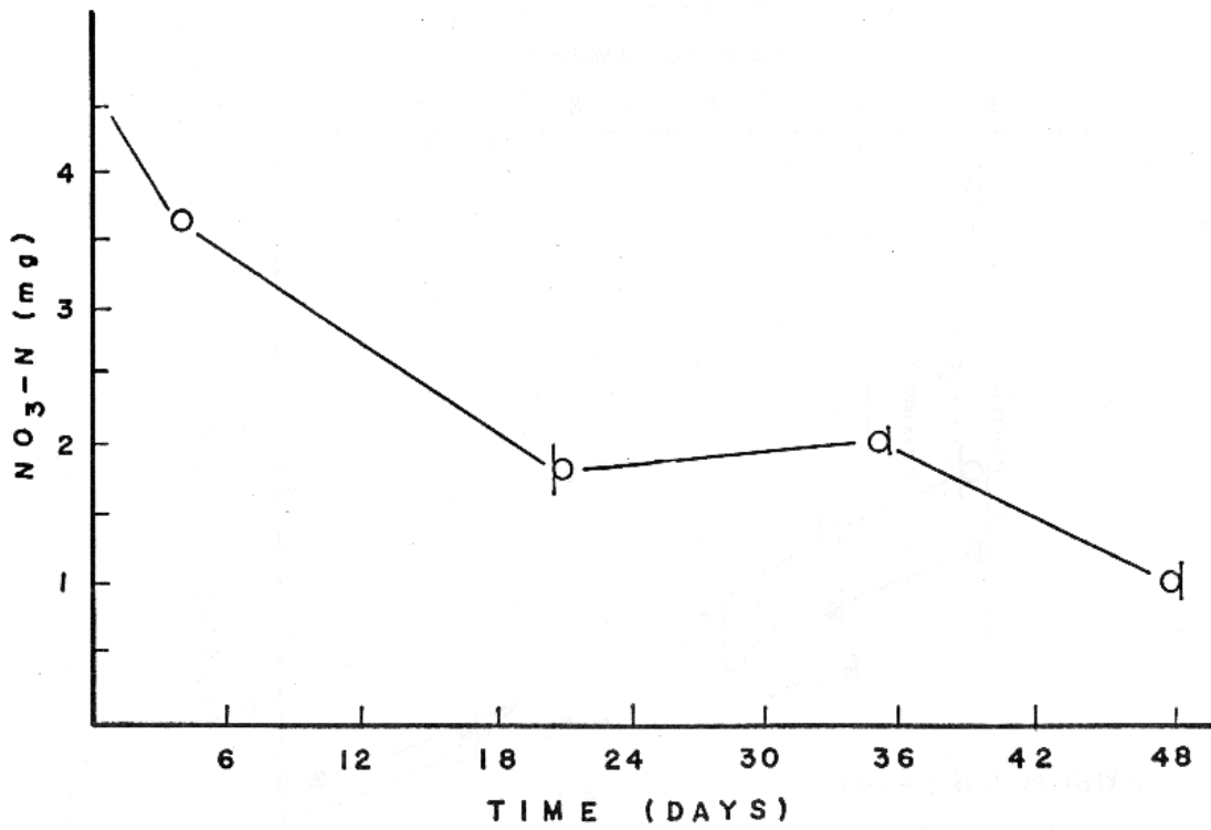
Figure 9: Changes in the concentration of nitrate-N (total of labelled and unlabelled) in columns incubated at 15°C for 48 days. Mean \pm SD.
