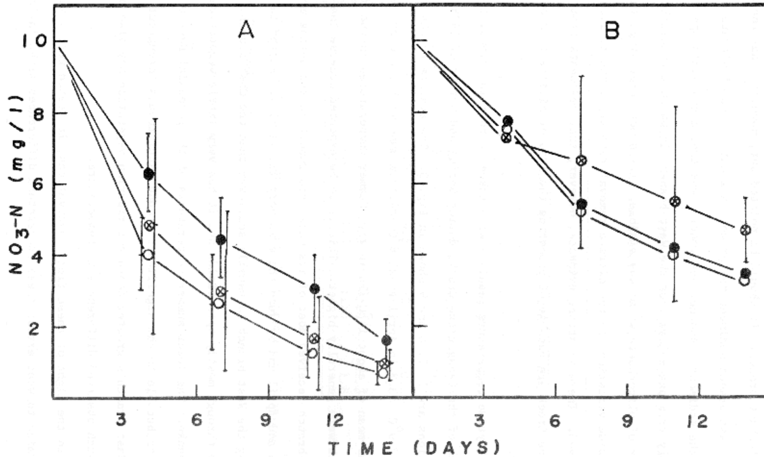
Figure 4: A. Changes in concentration of nitrate-N in water overlying sediment from two sites (⊗—⊗, ●—●) from the East branch and one site (O—O) from the West branch of Canagagigue Creek. Mean of 3 replicates ± SD.
