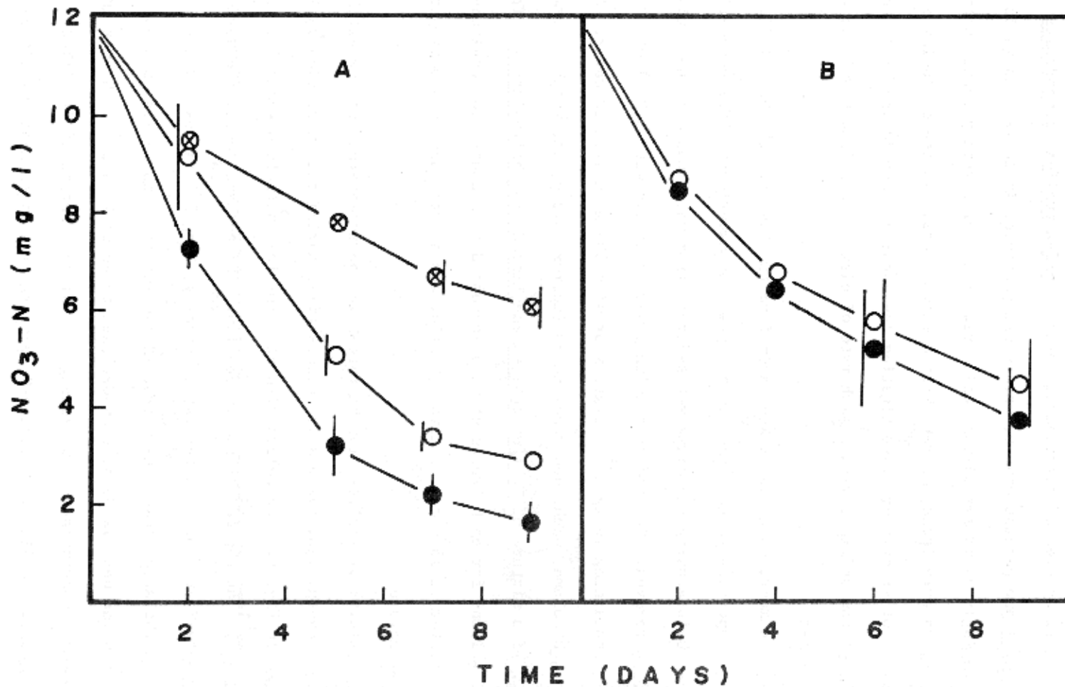
Figure 5: A. Changes in concentration of nitrate-N in water overlying Canagagigue sediment in columns maintained at 7°C (⊗—⊗), 15°C (O—O) and 22°C (●—●). Each point is the mean of 3 replicates \pm SD.
