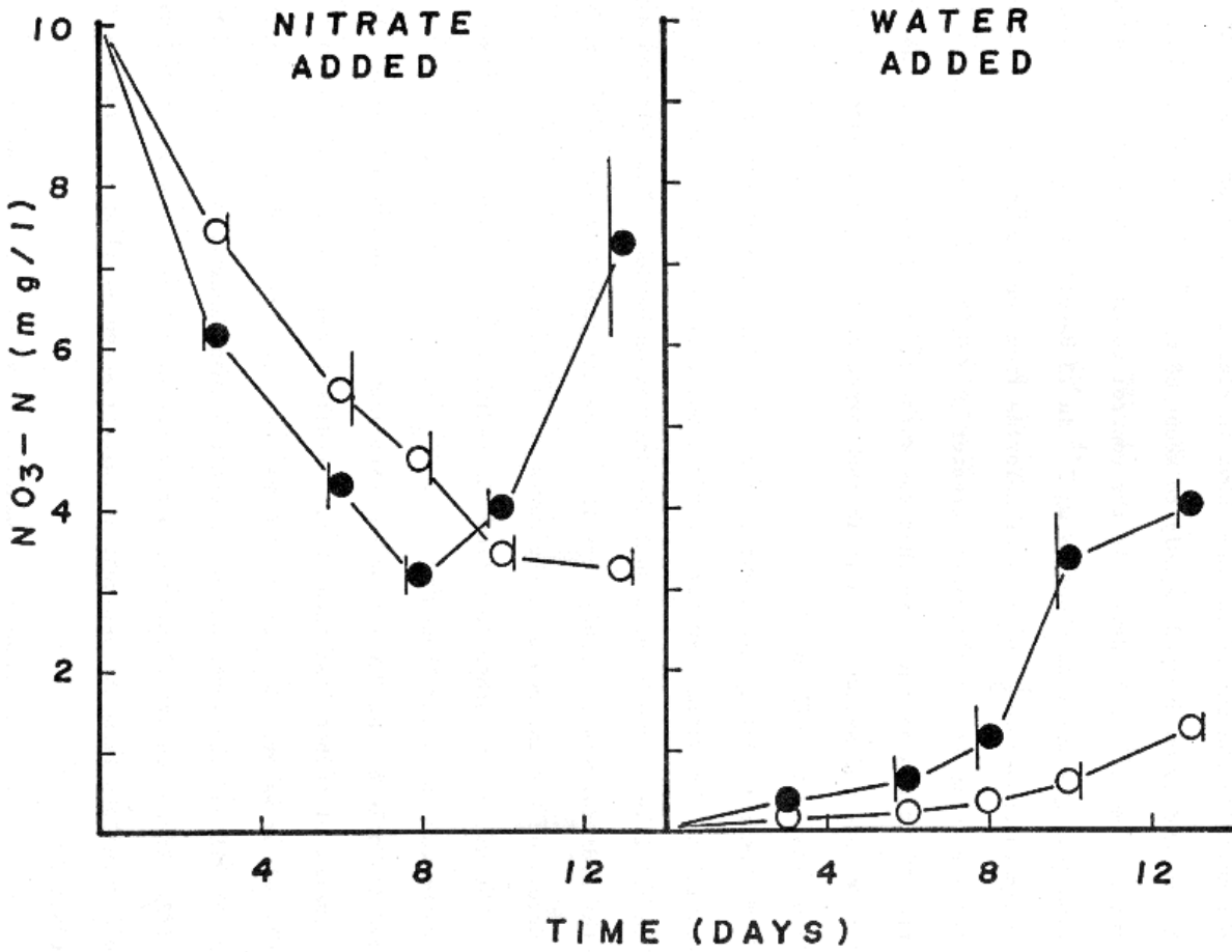
Figure 13: Changes in nitrate concentrations in Canagagigue columns incubated at 22°C for 13 days with (●—●) without (○—○) oligochaete worms. Mean \pm SD.
