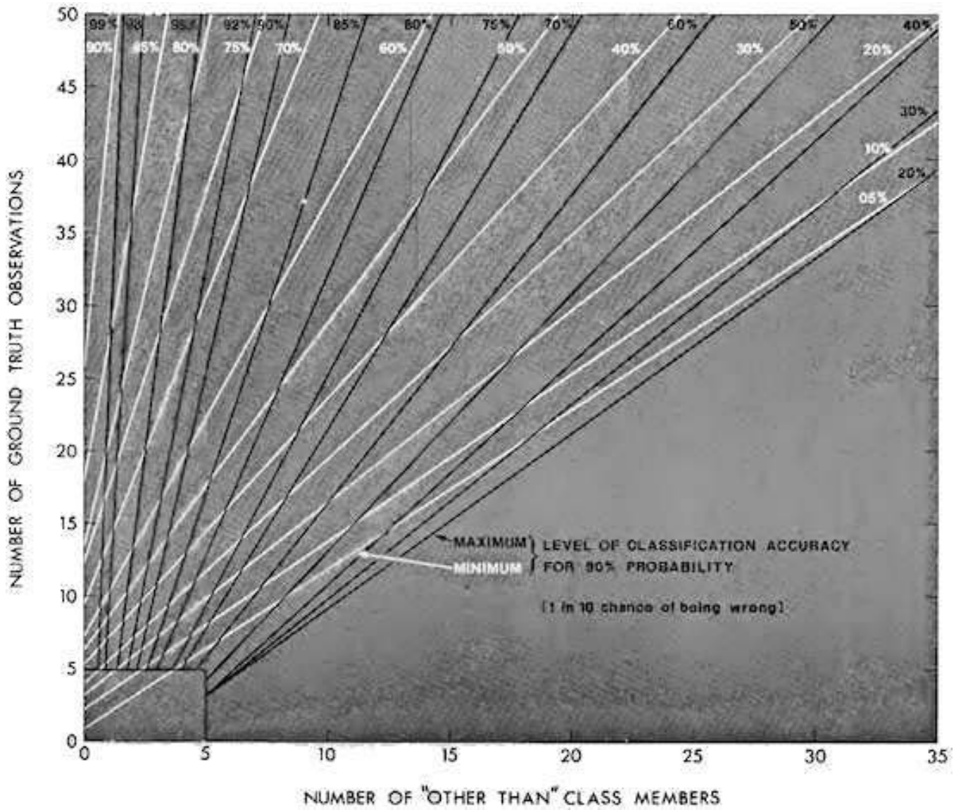
Figure 2. Arnold's Binomial Confidence. Limit Graph for 0 to 50 Samples.
