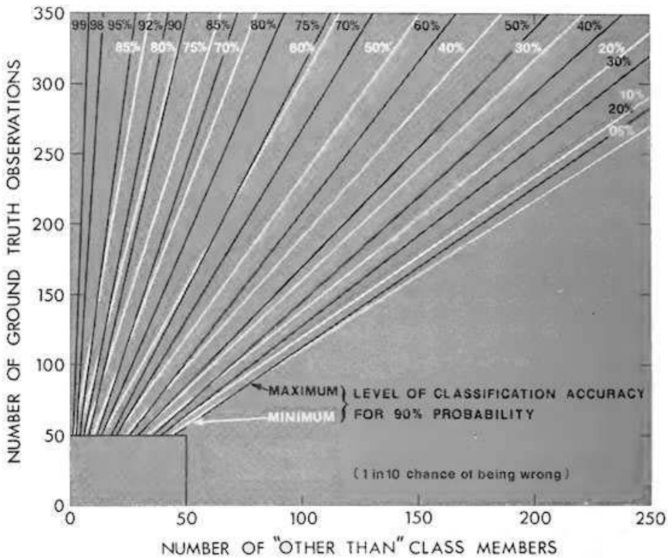
Figure 3. Arnold's Binomial Confidence. Limit Graph for 50 to 350 Samples.
