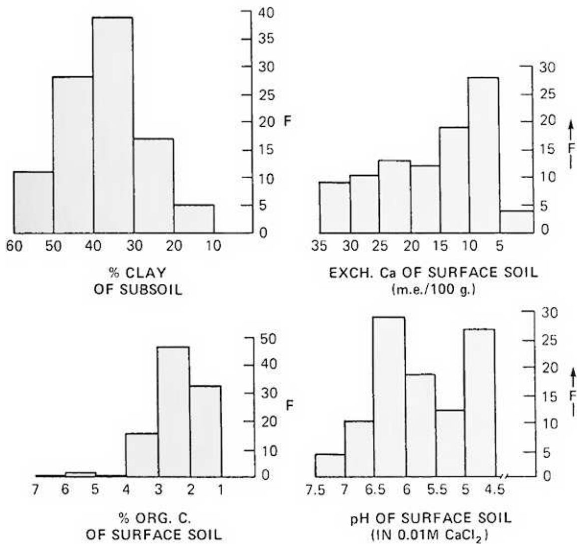
Figure 4. Frequency Distribution of a few Selected Soil Properties of Dalhousie Map Unit.
