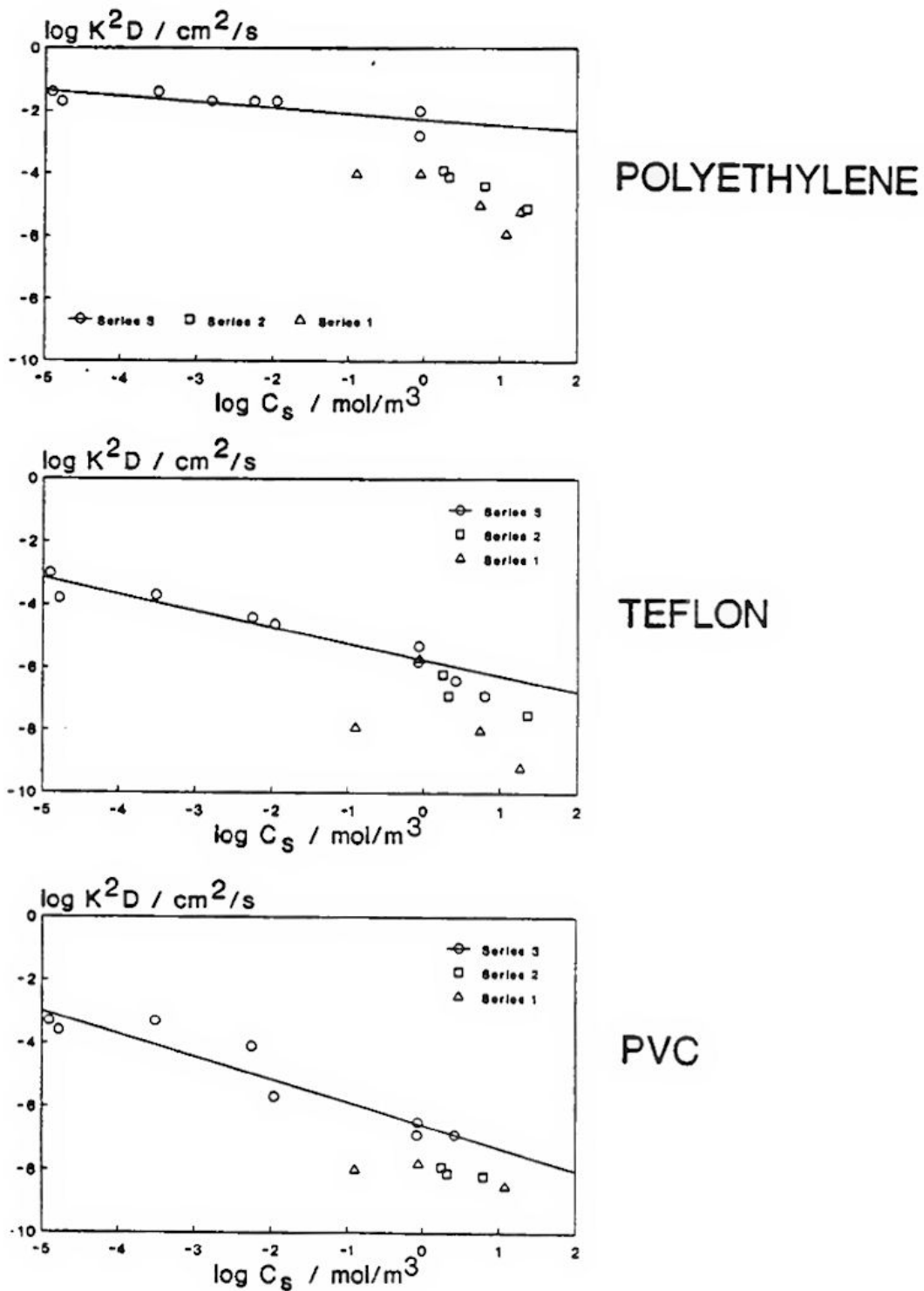
Figure 2. Log K^2D versus \log C_s plots for polyethylene, teflon, and rigid PVC. Series 1 and 2 data are for the low molecular weight halogenated and aromatic hydrocarbons, respectively. Series 3 data are for the chlorobenzenes and PCBs presently investigated. The regression lines for Series 3 data are also indicated.
