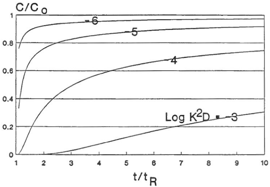
Figure 3. Breakthrough curves calculated by eq. 5 for various values of \log K^2D with t_R = 29.7 s and a = 0.0794 cm.
