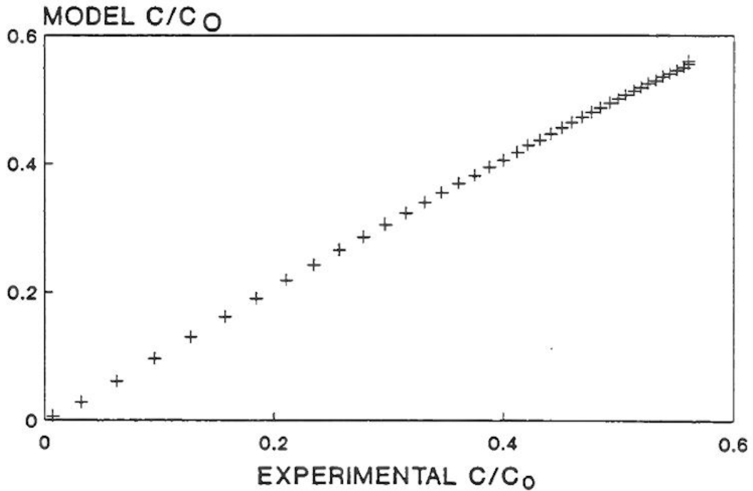
Figure 4. Parity plot for a breakthrough curve for ethylbenzene vapour in a 1/16" I. D. teflon tubing.
