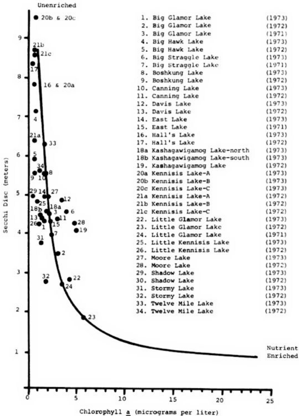
Figure 3: The relationship between Secchi disc and chlorophyll a for lakes in the Haliburton Highlands region of Ontario which have 2 or 3 consecutive years of data. Values for each lake are based on means of values collected during the summers of 1973 and 1972 and/or 1971.
