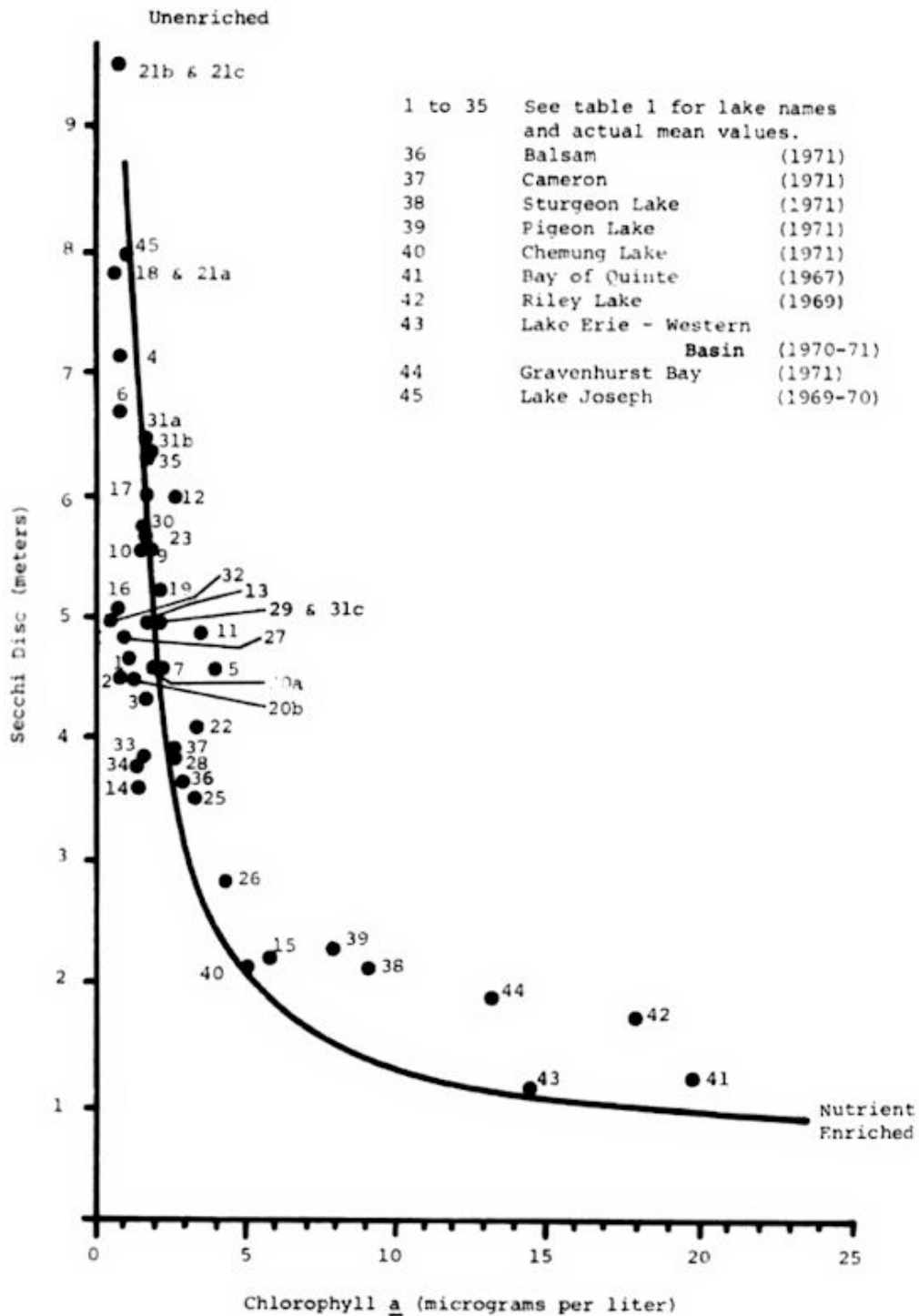
Figure 2: The relationship between Secchi disc and chlorophyll a for thirty-five lakes in the Haliburton Highlands region of Ontario. Values for each lake are based on means of values collected during the summer of 1973. Also, information from a number of other lakes is included as an indication of the relative status of lakes in the study area.
