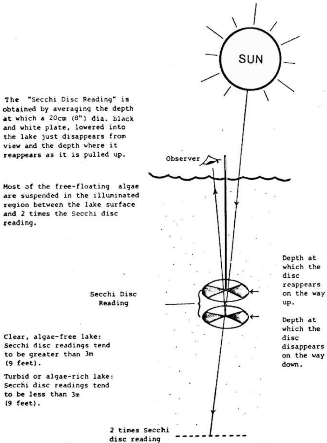
Figure 1: Diagram illustrating the use of a Secchi disc to measure water clarity.
