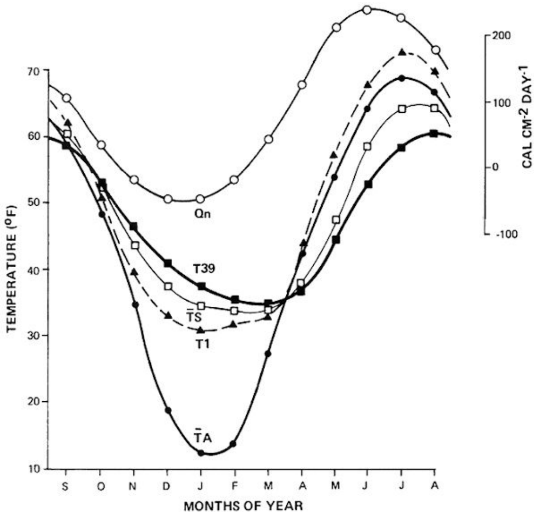
Fig. 1. Mean annual cycles of soil and air temperatures ( T_1 , T_{39} , \bar{T}_s , \bar{T}_a ) and net radiation ( Q_n ).
