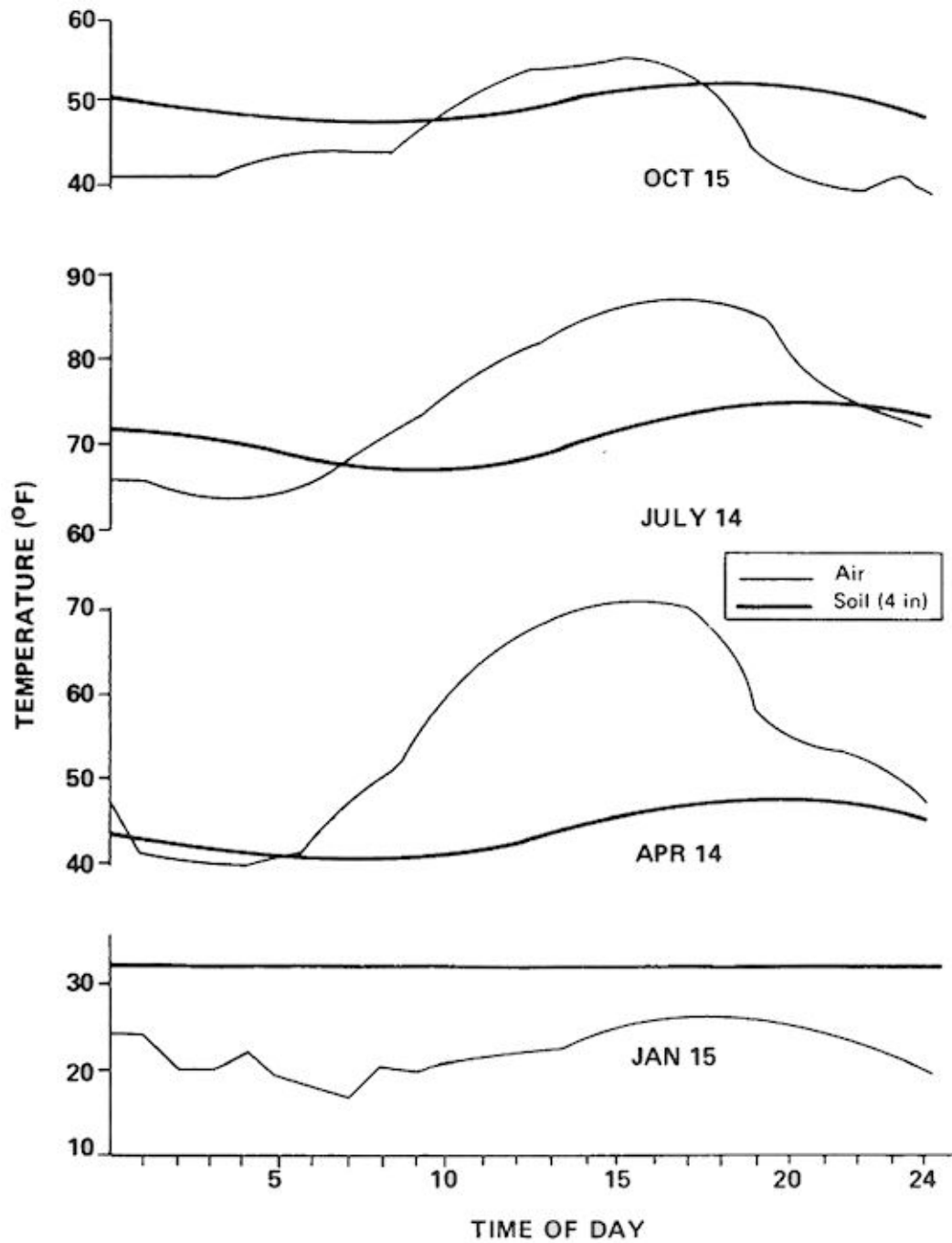
Fig. 3. Daily cycles of soil and air temperatures at Ottawa during four representative sunny days of 1970.
