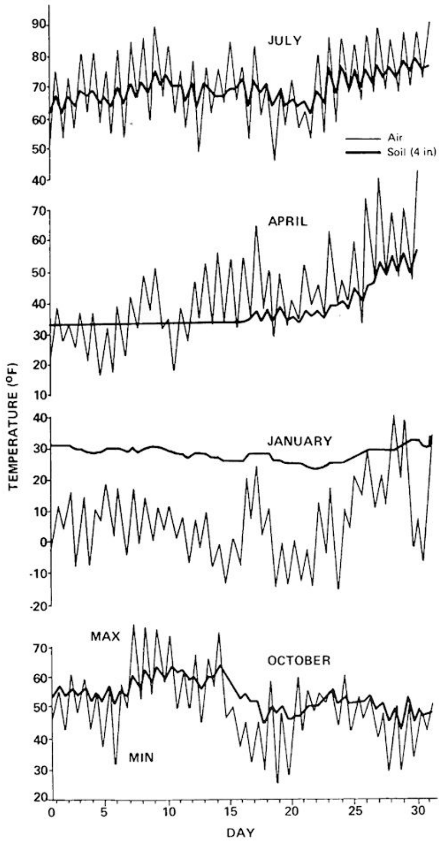
Fig. 4. Course of daily soil and air temperatures at Ottawa during four representative months of 1970.
