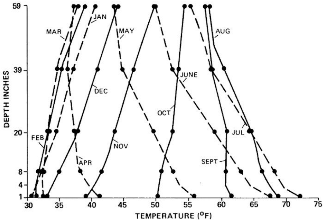
Fig. 2. Monthly soil temperature profiles.
