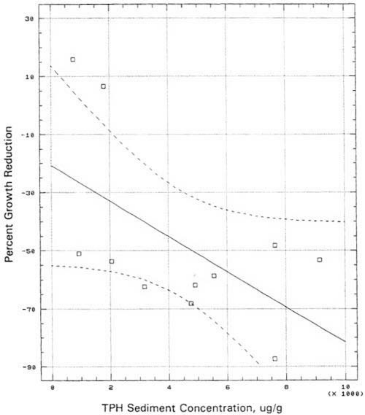
FIGURE 6. Regression Analysis of Midge 10-d Percent Growth Reduction on Bulk Sediment TPH Concentration for 1995.
