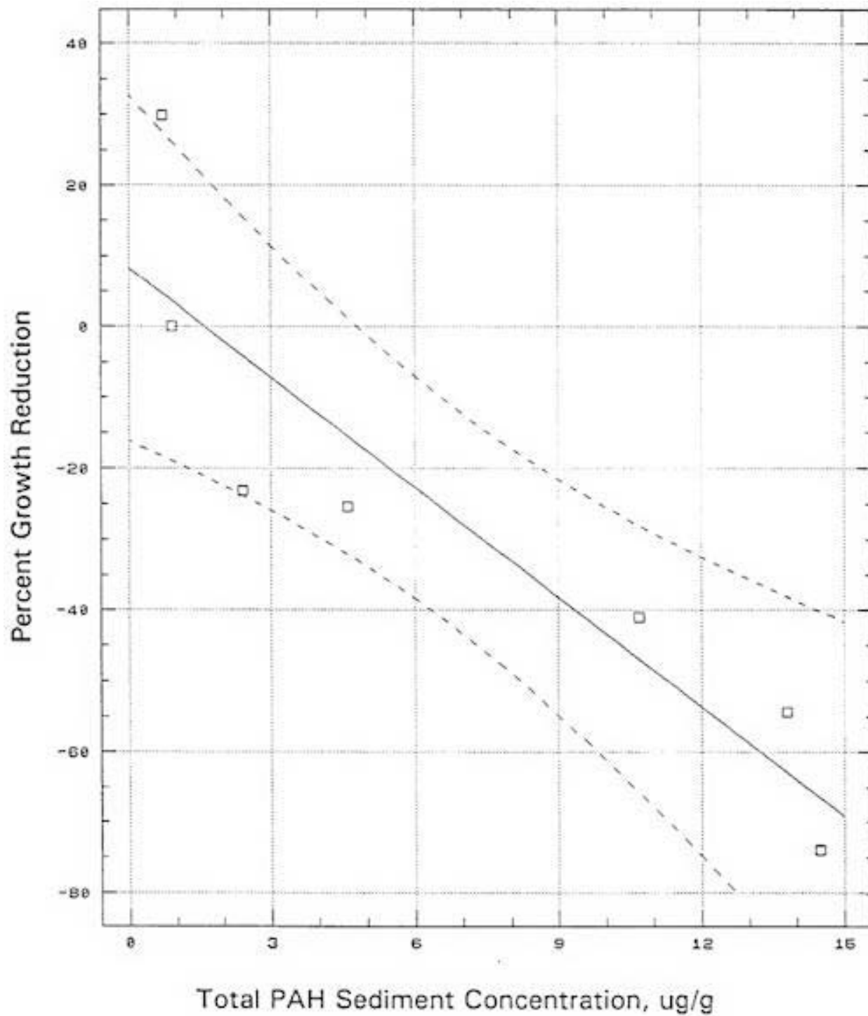
FIGURE 5A. Regression Analysis of Midge 10-d Percent Growth Reduction on Bulk Sediment total PAH Concentration for 1992.
