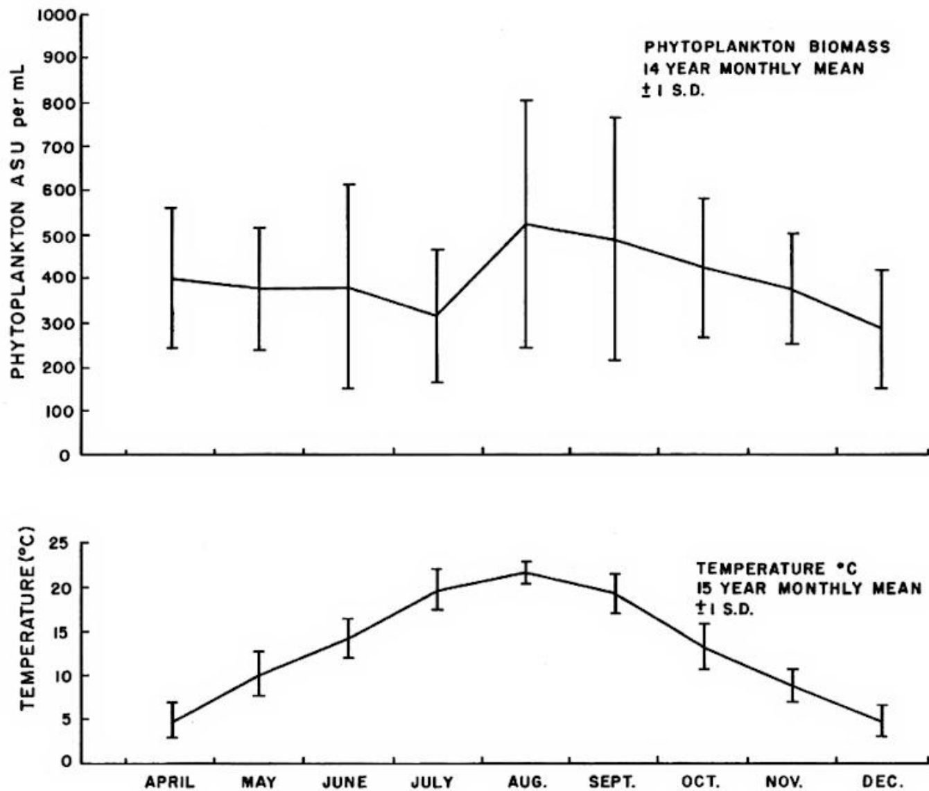
FIGURE 2. Seasonal Phytoplankton Abundance (14 yr. monthly) in the photic zone expressed as A.S.U./mL and Water Temperature (°C, 15 yr. monthly \bar{x} ) at 2 m depth from April to Dec. 1969-1983 at seven stations, Nanticoke, Lake Erie.
