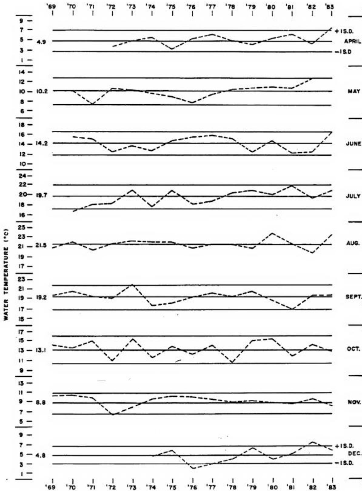
FIGURE 5. Temperature data — Differences between the 15 yr. average condition (heavy line — °C ± 1 S.D.) and the monthly mean for each year (dashed line) from 1969 to 1983 at seven stations, Nanticoke, Lake Erie.
